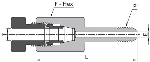
20D Series Tube Fittings to Medium Pressure Cone & Thread Tubing
