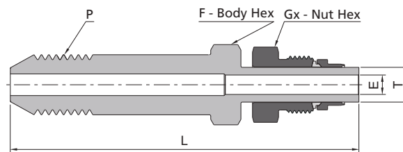
Medium Pressure Cone & Thread Tubing to Split Male 20D Series Tube Fittings ①
