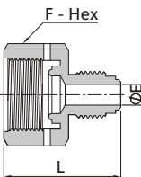
Reducing Adapter
